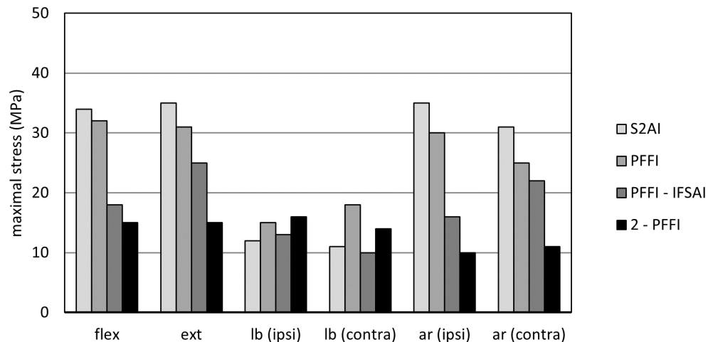
Figure 4. Maximal stresses in the left implants placed in an S2 alar-iliac (S2AI), trajectory predicted for 4 instrumented configurations (S2AI, PFFI, PFFI-IFSAI, and 2-PFFI). “flex”: flexion; “ext”: extension; “lb (ipsi)”: lateral bending in the ipsilateral direction (the same side of the implant of interest); “lb (contra)”: lateral bending in the contralateral direction; “ar (ipsi)”: axial rotation in the ipsilateral direction (the same side of the implant of interest); “ar (contra)”: axial rotation in the contralateral direction. Refer to Table 1 for model descriptions and abbreviations.
